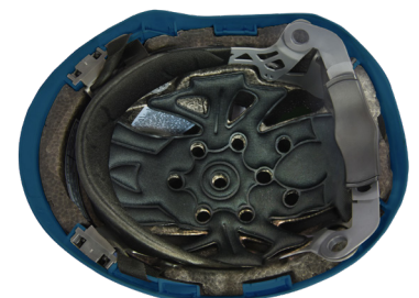
Interior Suspension
