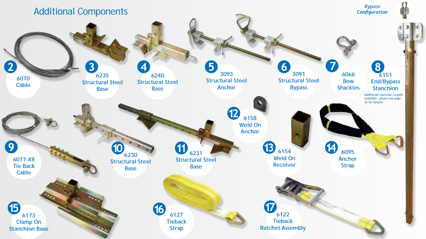
1 6310 Horizontal Lifeline System Components
