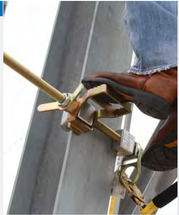
*Must be used with the BlackMax™ shock absorber when anchored at foot level
