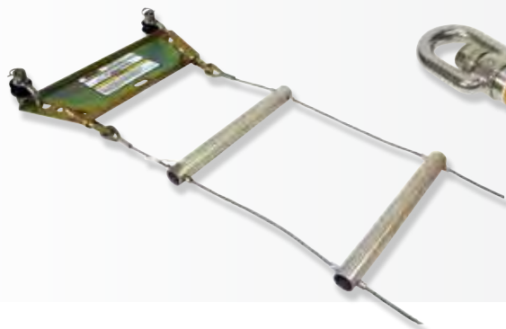
5230 - 30' (9.1m) Wire Rope Ladder for HLL rescue (bracket not included)
